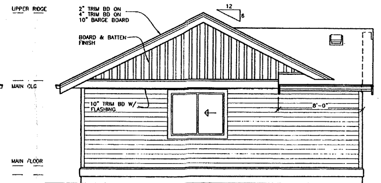
LEFT ELEVATION
