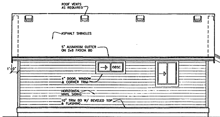
REAR ELEVATION
